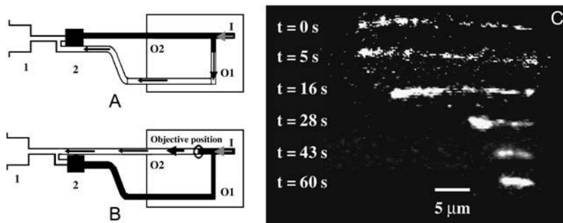
FIGURE 1 Schematic of the experimental apparatus. Syringe pump (1), electro-valve (2), inlet channel (I), outlet channel 1 (O1), and outlet channel 2 (O2). (A) Biological samples are aspirated in microchannel O1 until the concentration is homogeneous at the T-junction. (B) The electrovalve switches the aspiration to channel O2 where the objective is positioned. (C) Example of compaction of an individual DNA molecule in time in the presence of 2 ng/μL of native histones.
